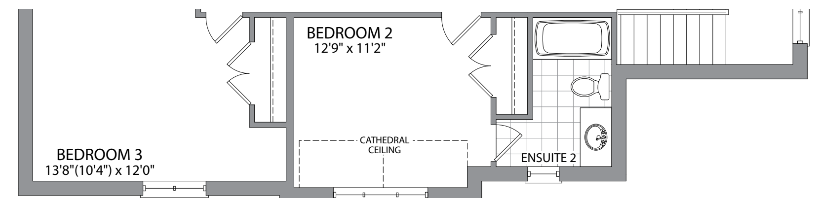
PARTIAL SECOND FLOOR ELEVATION B
