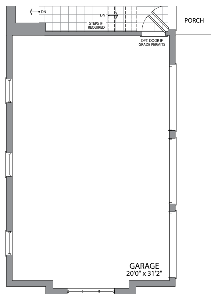
PARTIAL GROUND FLOOR WITH OPTIONAL RETREAT ELEVATION B
