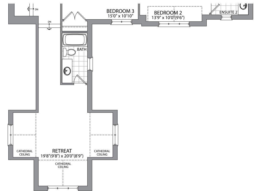
PARTIAL SECOND FLOOR WITH OPTIONAL RETREAT ELEVATION B
