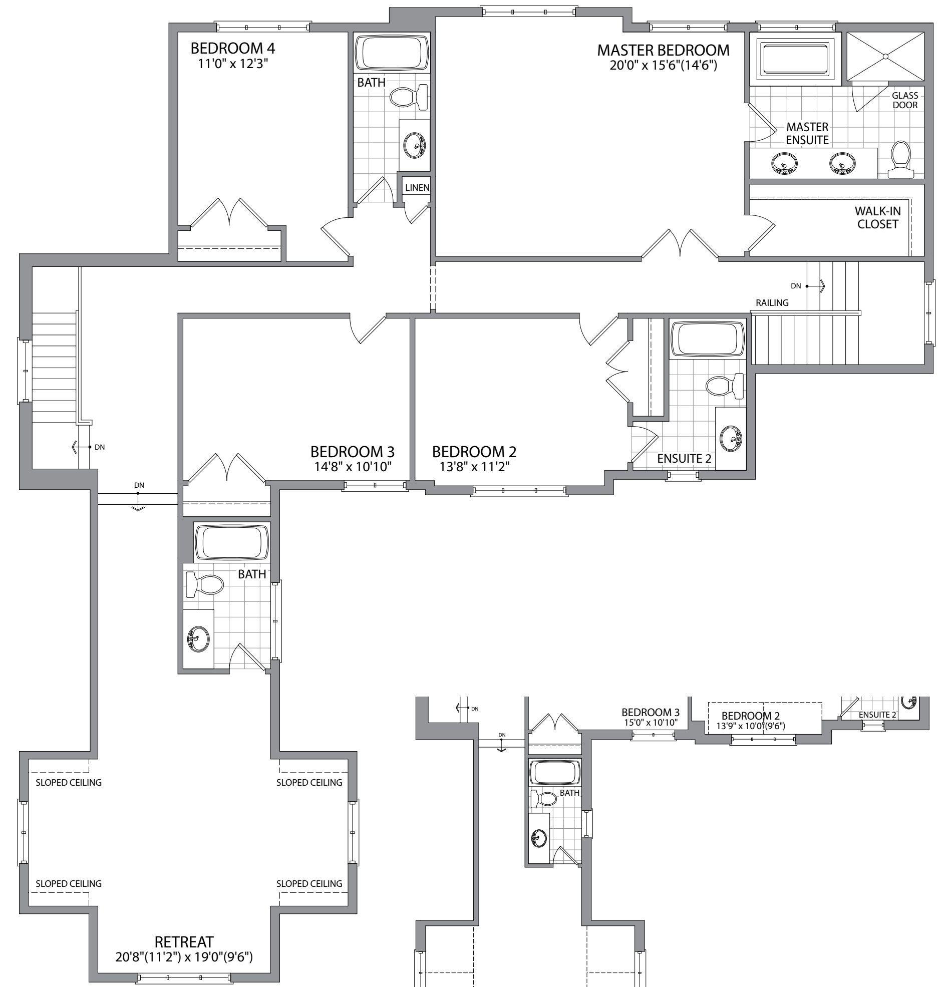
SECOND FLOOR WITH OPTIONAL RETREAT ELEVATION A & B
