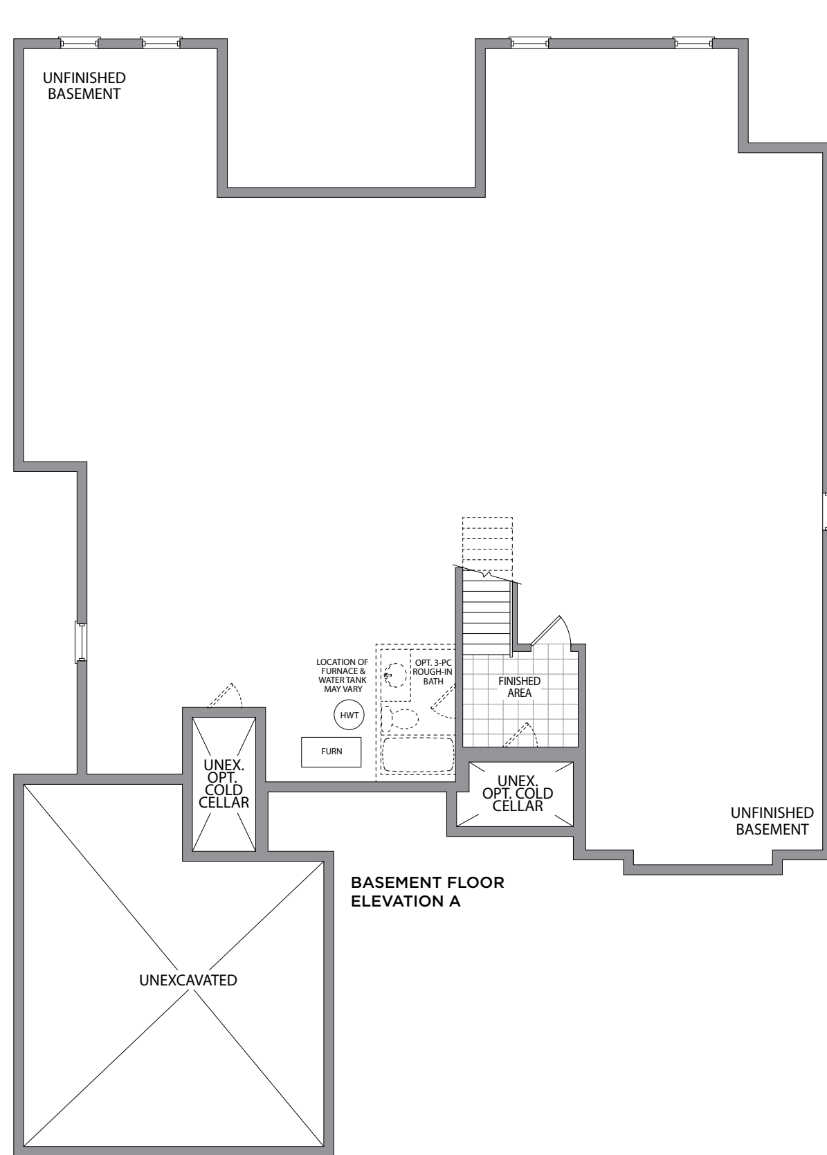
ELEVATION A - 2,596 SQ. FT.
