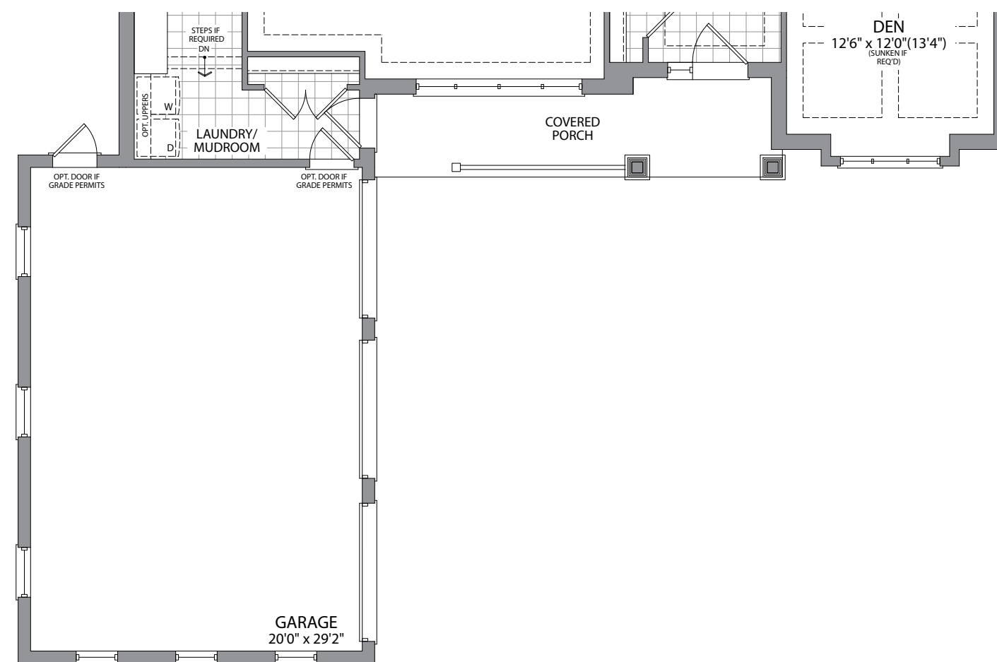
PARTIAL GROUND FLOOR ELEVATION B
